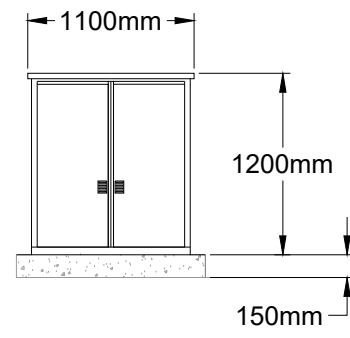
RMU FRONT VIEW
