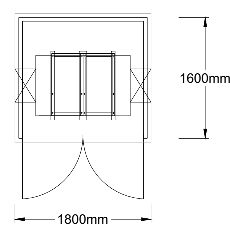
RING MAIN UNIT (RMU) ENCLOSURE PLAN VIEW
