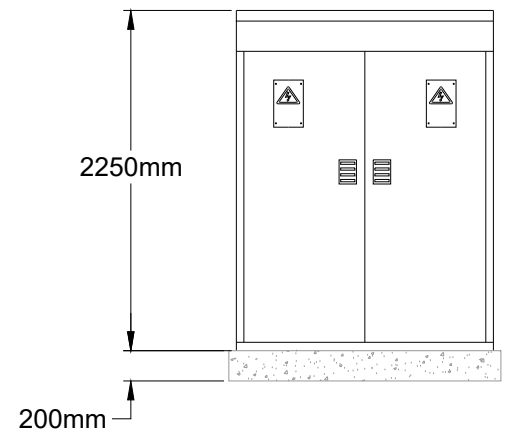
RMU FRONT VIEW
