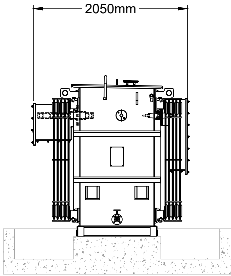
SIDE ELEVATION
