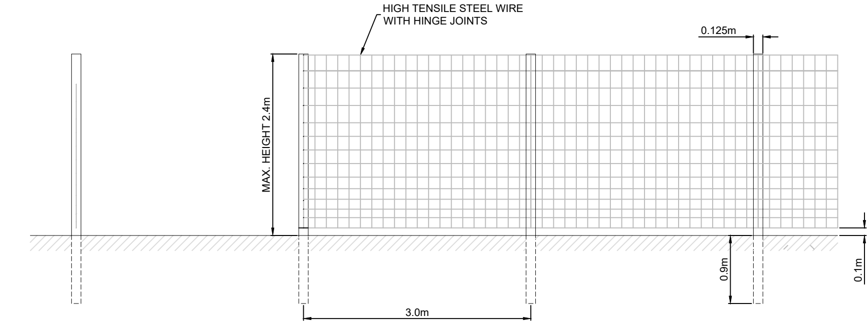
DEER FENCE END ELEVATION
