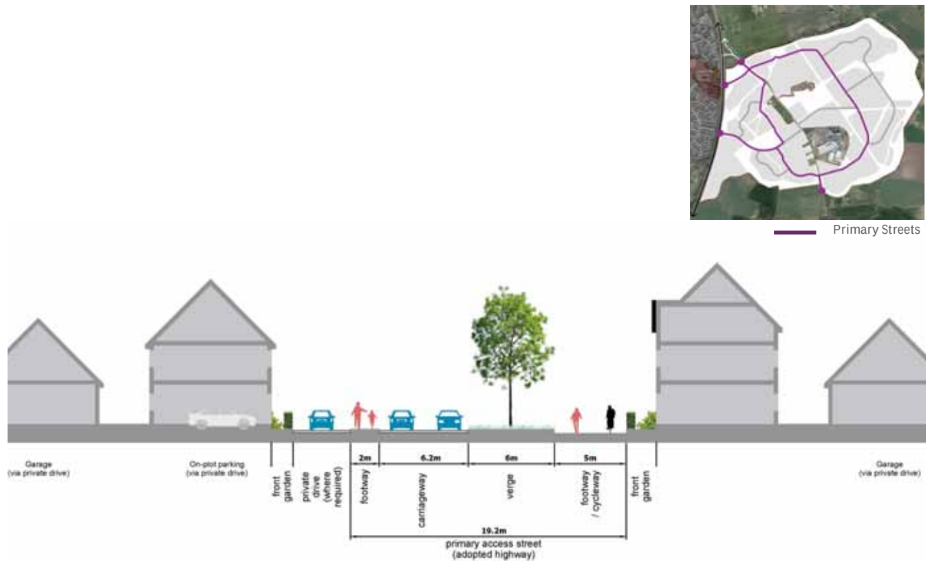
Figure 36. Indicative Primary Street Section
