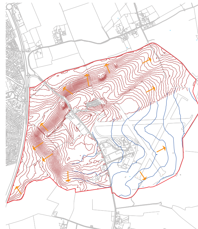
Figure 10. Site Contour Plan
