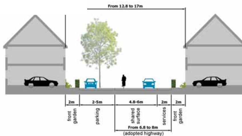
Figure 40. Indicative Secondary Street Section
