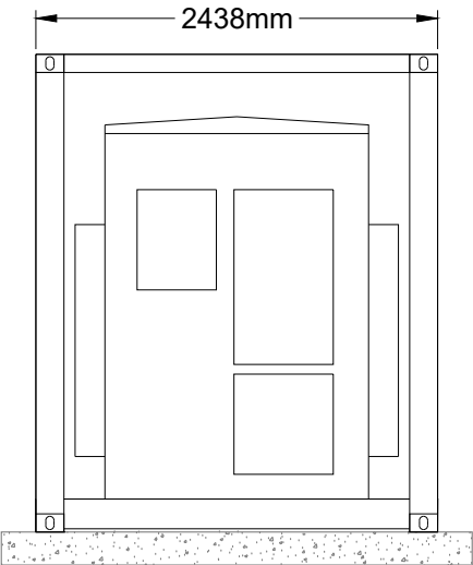
SIDE ELEVATION - 1
