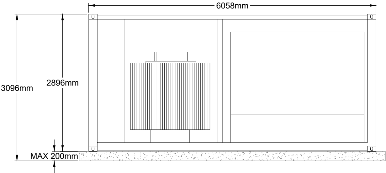
BACK ELEVATION
