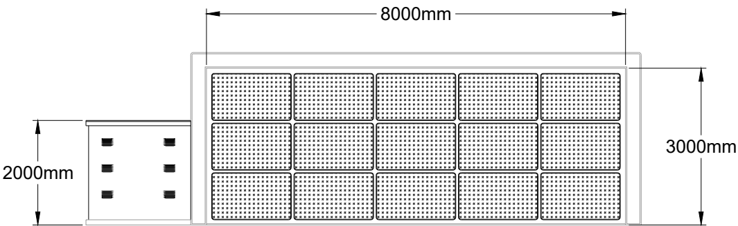
SIDE ELEVATION - 1
