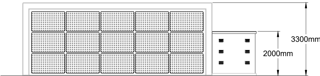
SIDE ELEVATION - 2
