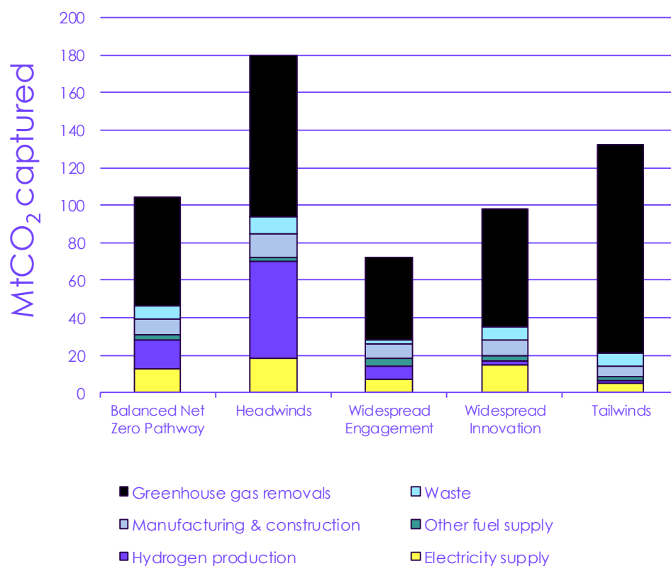
Figure 2.14 Total amount of CO 2 captured in 2050 in the scenarios
