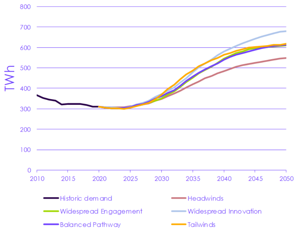
Figure 3.4.d Electricity demand across the exploratory scenarios (2010-50)
