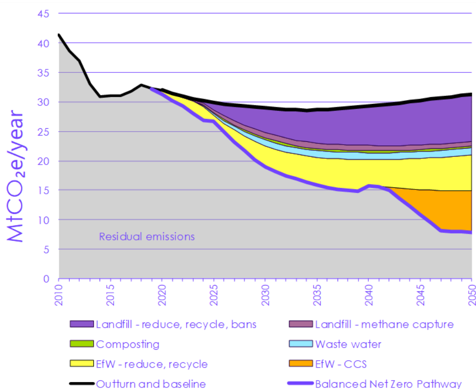
Figure 3.9.a Sources of abatement in the Balanced Net Zero Pathway for the waste sector
