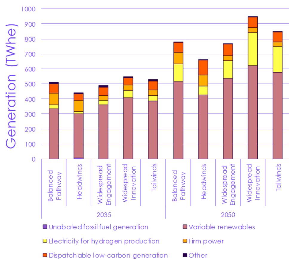
Figure 3.4.e Illustrative generation mix for the exploratory scenarios (2035 and 2050)
