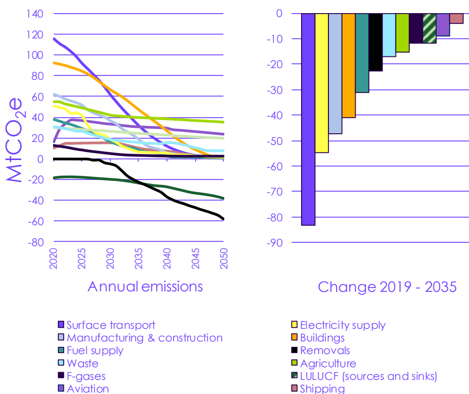
Figure 2.4 Sectoral emissions under the Balanced Net Zero Pathway
