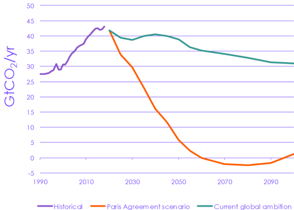
Figure 7.4 Global CO 2 emissions in a 'leadership-driven' Paris Agreement scenario and under current global ambition
