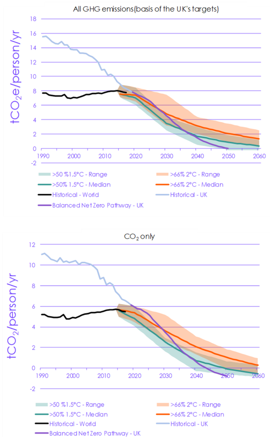
Figure 7.2 Global emissions pathways (per person) consistent with the Paris Agreement
