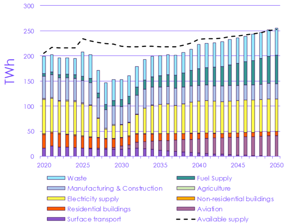
Figure 3.5.d Bioenergy and waste use in the Balanced Net Zero Pathway
