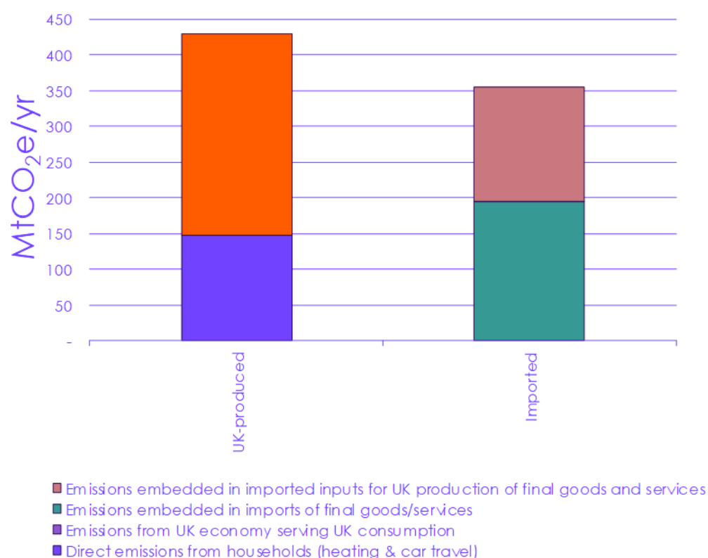
Figure 7.6 Decomposition of UK consumption emissions in 2016
