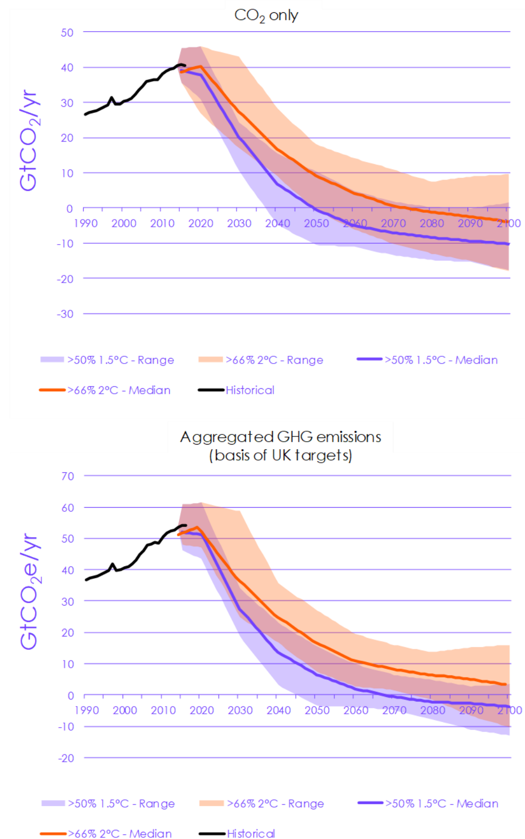
Figure 8.1 Global emissions pathways consistent with the Paris Agreement
