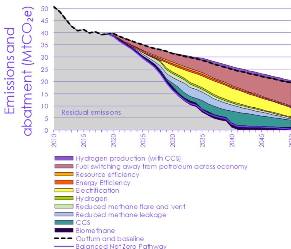
Figure 3.5.a Sources of abatement in the Balanced Net Zero Pathway for the fuel supply sector
