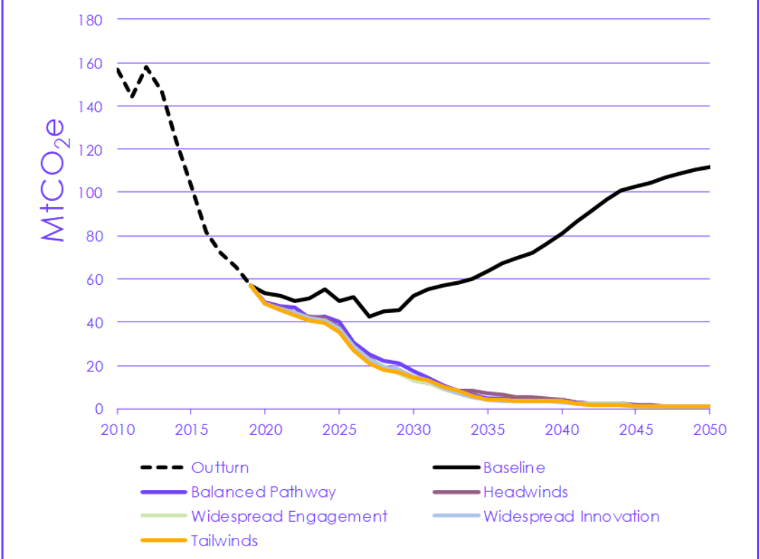
Figure 3.4.f Emissions pathways for electricity generation (2010-50)
