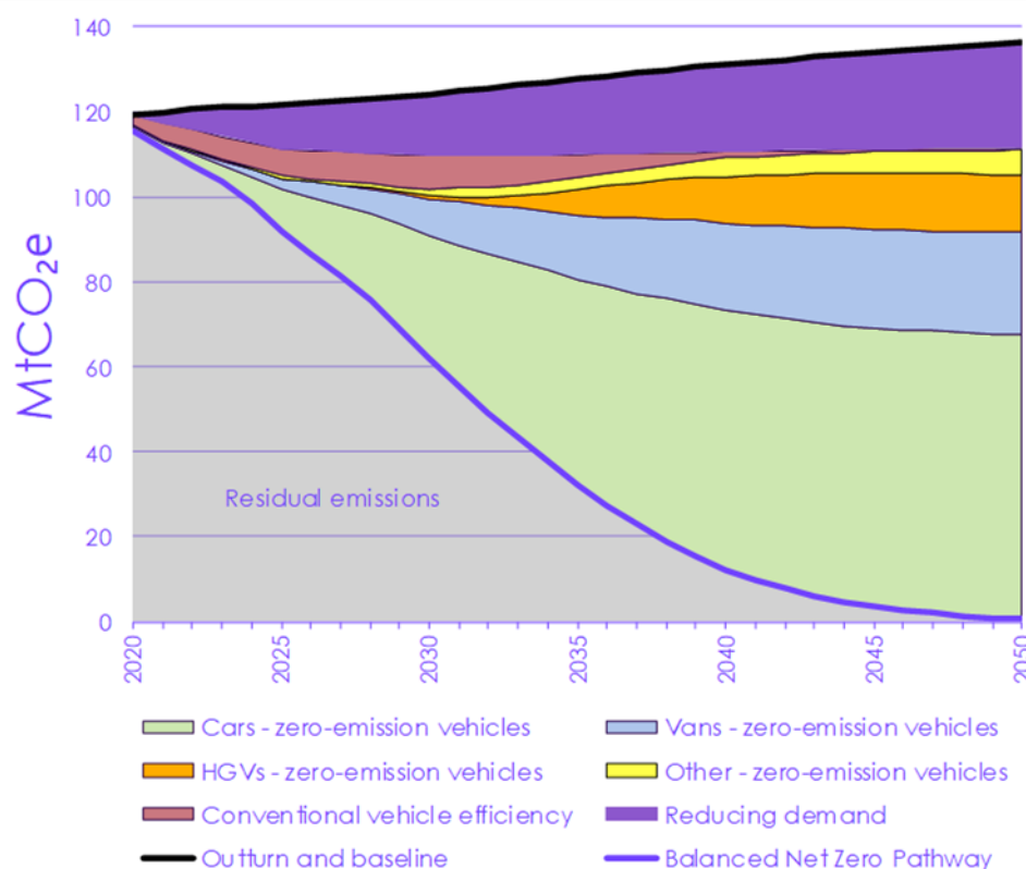
Figure 3.1.a Sources of abatement in the Balanced Net Zero Pathway for the surface Transport sector
