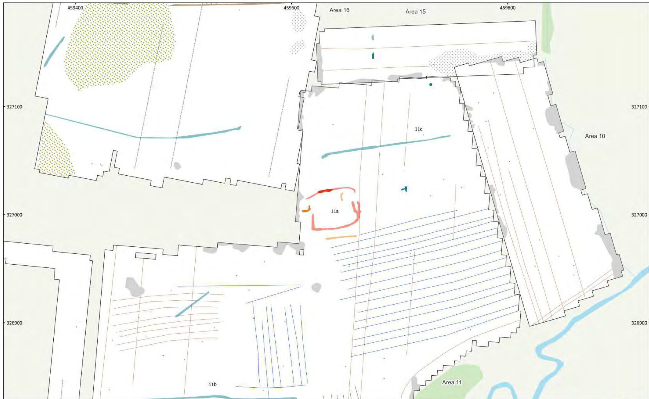
MSSK1600 - Old Wood Energy Park, Willoughby, Nottinghamshire Figure 36 - Magnetic Interpretation (Areas 10, 11 & 15) 1:1,500 @ A3 Copyright Magnitude Surveys Ltd 2023 Contains Ordnance Survey data © Crown Copyright and database right 2023
